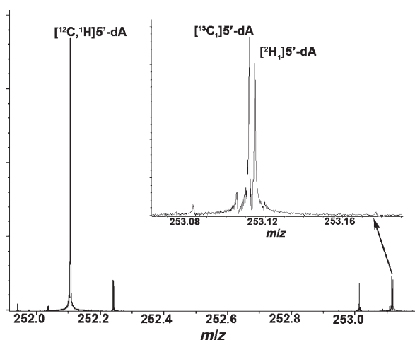
Figure 1. High-resolution electrospray (positive-ion mode) ICR MS of 5'-dA isolated from glutamate mutase after reaction with [ ^2\text{H}_1 ]methylaspartate for 36 ms. The peaks due to ^{13}\text{C}, ^2\text{H} -labeled and unlabeled 5'-dA are indicated. Inset: Expansion of the region around 253.115 amu showing the ^{13}\text{C} -labeled and ^2\text{H} -labeled ions clearly resolved (the small peak at 253.108 is due to natural-abundance [ ^{15}\text{N} ]5'-dA).
