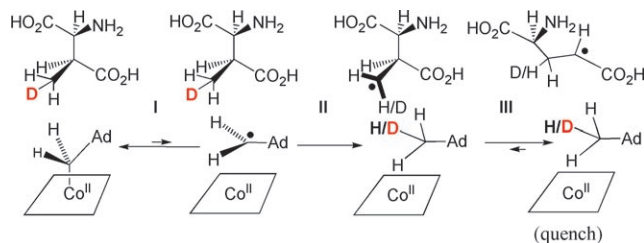
Scheme 2. Measurement of intrinsic KIE by intramolecular isotope competition using [ 2 H] 1 -methylaspartate. Isotopic discrimination occurs in step II, and rapid rearrangement of methylaspartyl radical to glutamyl radical (step III) prevents scrambling of the deuterium between substrate and coenzyme on the short time scales employed in the experiment.
